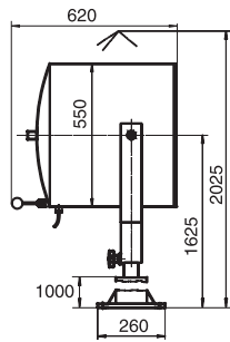
NHS550B Gewicht/ weight: 26.7 kg
